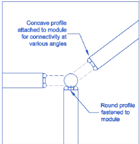
A3 Horizontal detail @ module connection
