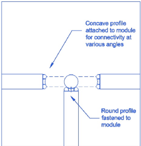
A2 Horizontal detail @ module connection
