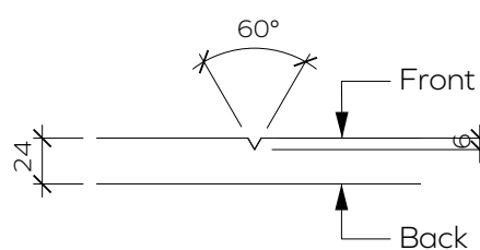
V-cut Detail
