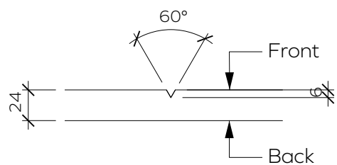
V-cut Detail
