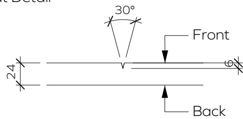
V-cut Detail
