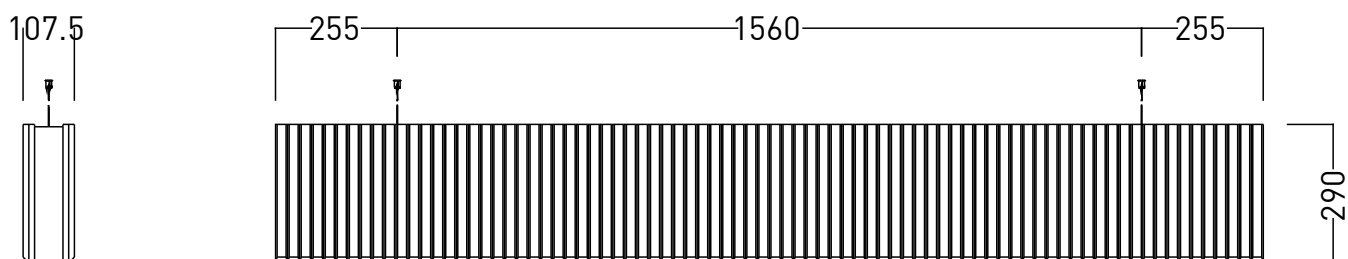
SIDE ELEVATION
