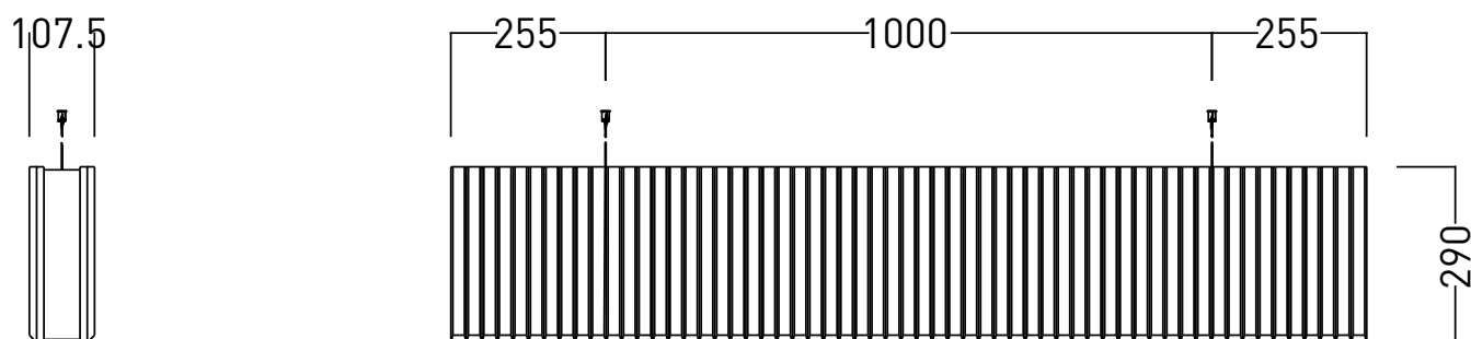
SIDE ELEVATION
