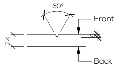
V-cut Detail
