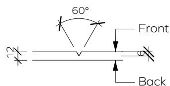
V-cut Detail
