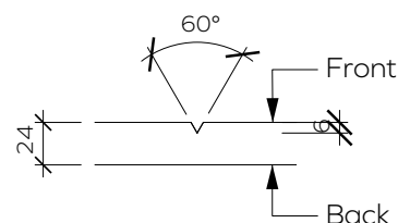
V-cut Detail
