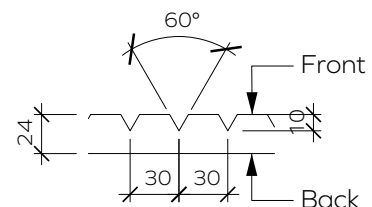
V-cut Detail
