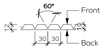
V-cut Detail
